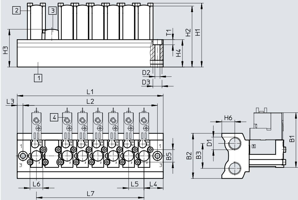
[1] Connection block [2] Retaining bracket [3] Blanking plate [4] Valves
