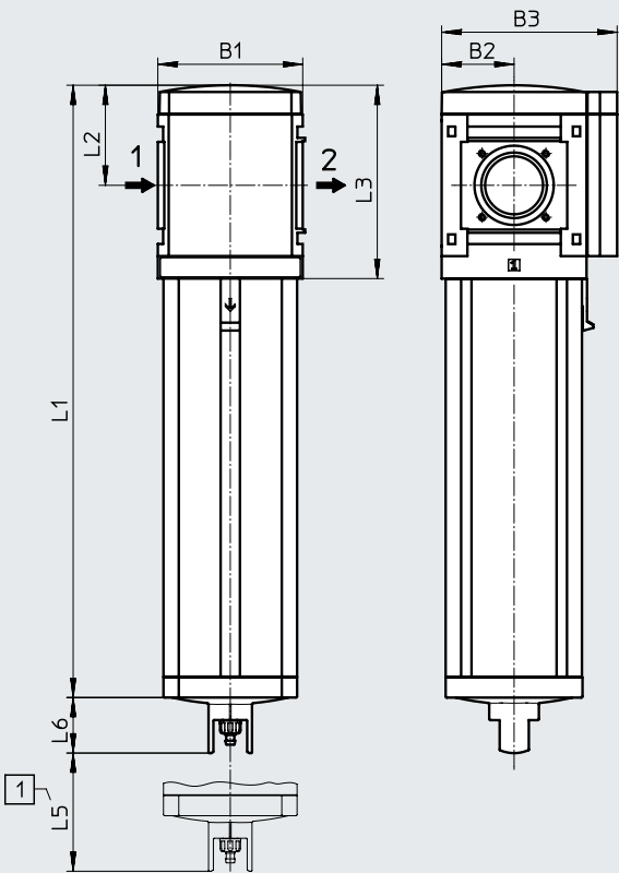
[1] Installation dimension → Flow direction
